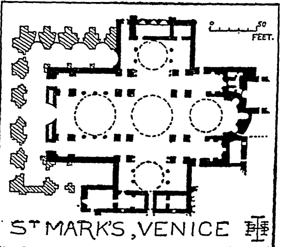
FIGS. 27 AND 28.—SECTION AND PLAN OF ST. MARK'S.
